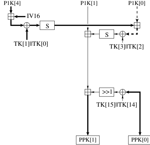
Figure 9: Part of Phase 2 needed to calculate TK[2], TK[3], TK[14], and TK[15].
